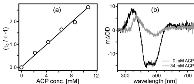
Figure 3. Stern–Volmer plot based on luminescence lifetimes ( \lambda_{\text{det}} = 615\text{ nm} ) of ca. 10^{-5}\text{ M} \text{Mo}(\text{CNAr}_3\text{NC})_3 in deaerated THF at 20^\circ\text{C} in presence of increasing concentrations of acetophenone (ACP). b) Transient absorption of ca. 10^{-5}\text{ M} \text{Mo}(\text{CNAr}_3\text{NC})_3 in the absence (black) and presence (gray) of 34\text{ mM} ACP. Excitation and detection was as described above. The disappearance of the bleach between 400 and 520\text{ nm} is caused by formation of the ACP radical anion ( \text{ACP}^- ); see text and pages S14–S16 in the Supporting Information.
