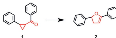
Scheme 1. Rearrangement of acyl cyclopropane ( 1 ) to 2,3-dihydrofuran ( 2 ) accomplished in 84\% yield through photoirradiation ( \lambda_{\text{exc}} = 455\text{ nm} ) of 5\% \text{Mo}(\text{CNAr}_3\text{NC})_3 in dry [\text{D}_6]\text{benzene} ( \text{TON} = 17 ).
