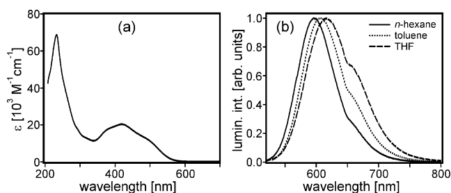
Figure 2. a) UV/Vis absorption spectrum of \text{Mo}(\text{CNAr}_3\text{NC})_3 in THF at 20^\circ\text{C} . b) Luminescence spectra in different solvents at 20^\circ\text{C} ( \lambda_{\text{exc}} = 500\text{ nm} ).
